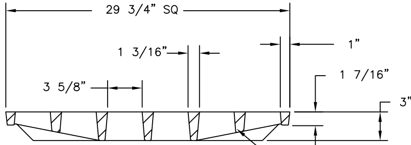
GRATE SECTION
